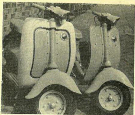
TINA FAIRING: Giving very much more weather protection to the Tina scooter rider, the new Blacknell Riviera fairing is seen here fitted (l).
