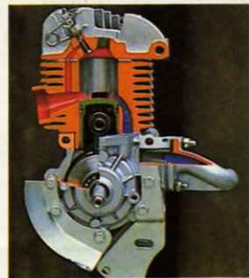
CUTAWAY OF AV10 ENGINE
