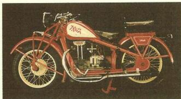
JAWA 500 OHV • Four stroke OHV single cylinder • Displacement 498.7 cc (bore and stroke 84×90 mm) • Engine power 13.2 kW • Forced feed dry sump lubrication • Three-speed gearbox in unit with engine, hand control • Rigid suspension rear wheel drive by propeller shaft with caliper brake • Duplex frame welded of steel stampings • Front fork with trailing link and quarter elliptic leaf spring suspension • Weight 175 kg • Maximum speed 95 km p.h. • Average fuel consumption 5 to 6 litres per 100 km
