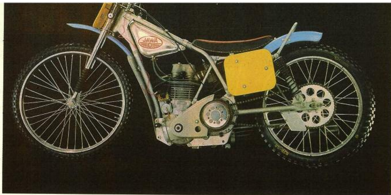
JAWA 500, Model 896 ● Four stroke air-cooled OHC single cylinder ● Displacement 496 cc (bore and stroke 85×87 mm) ● Engine power 48 kW at 8,600 r.p.m. ● Compression ratio 14 to 1 ● Four-valve cylinder head ● Total loss lubrication by double pump ● Two-speed gearbox ● Multiplate dry clutch ● Simple frame welded of steel tubes ● Pivoted rear fork with two oil damped suspension units ● Telescopic front fork ● Weight 93 kg ● Maximum speed and fuel consumption not indicated
