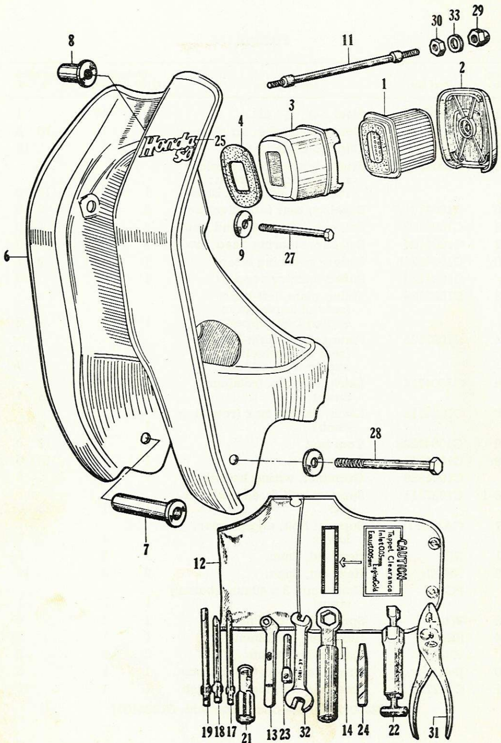
FRONT LEGSHIELD — AIR CLEANER — TOOLKIT
