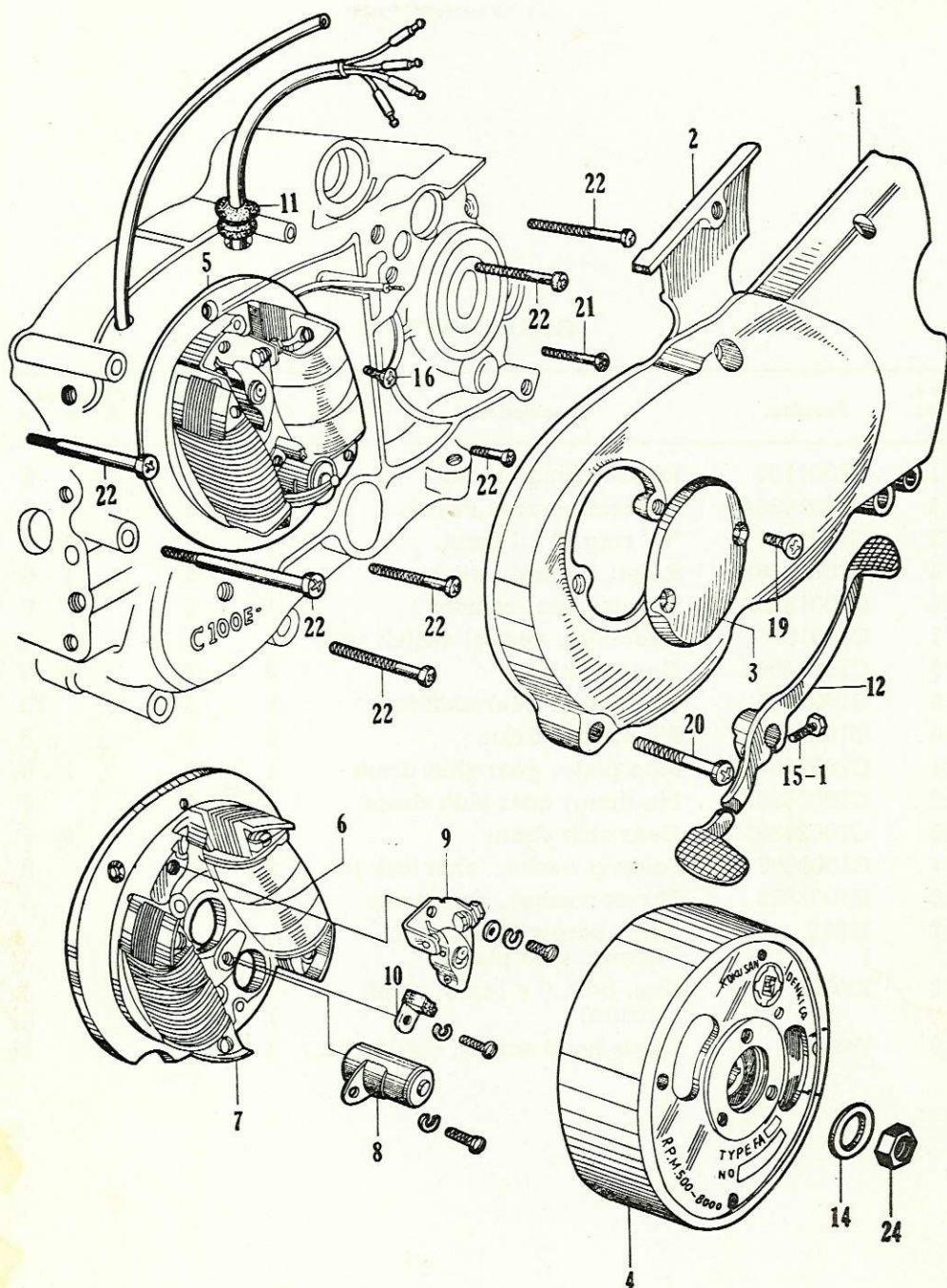
CONTACT BREAKER — LEFT-HAND CRANKCASE COVER
