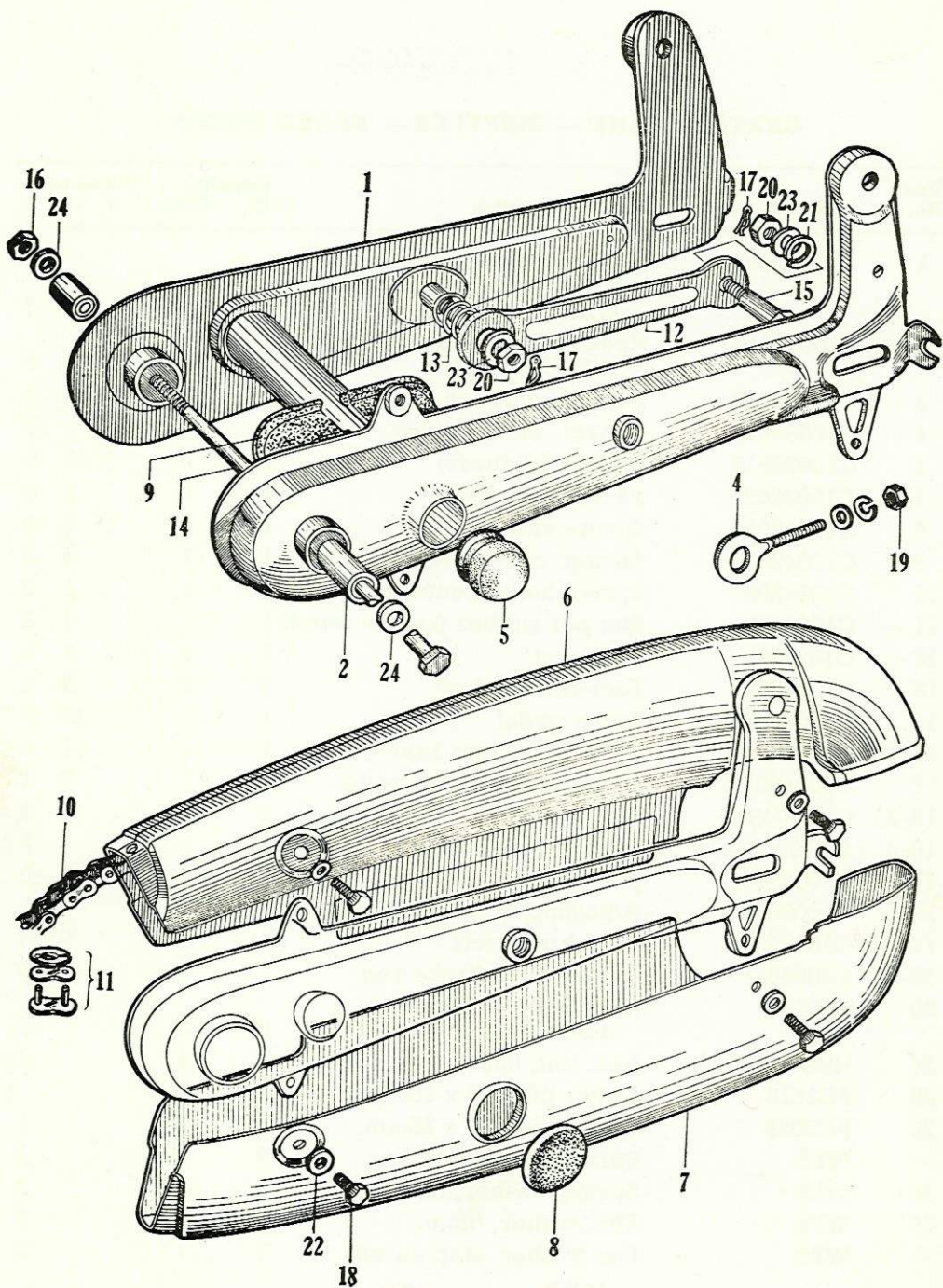
REAR FORK — CHAIN CASE
