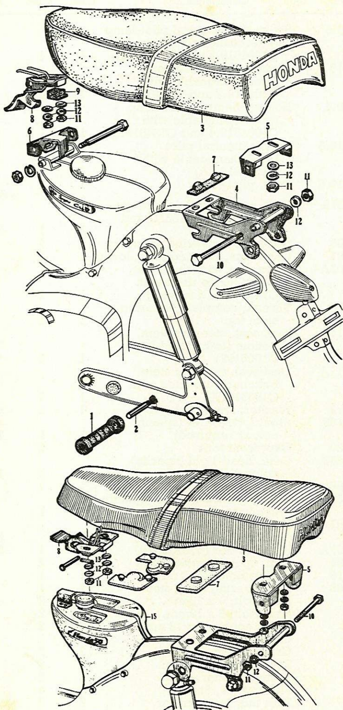
FUEL TANK — DUAL SEAT
