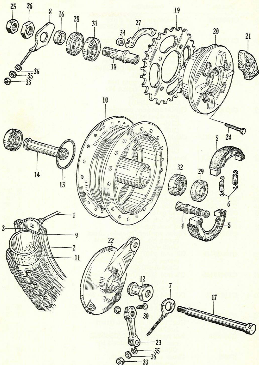
REAR WHEEL
