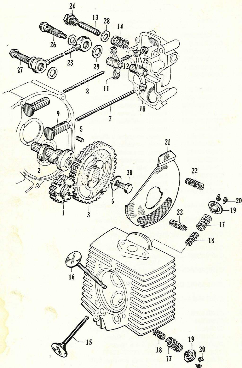
CAMSHAFT — TIMING GEAR — VALVES — OIL FEED PIPE
