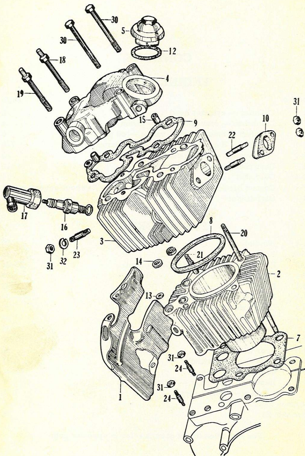
CYLINDER — CYLINDER HEAD
