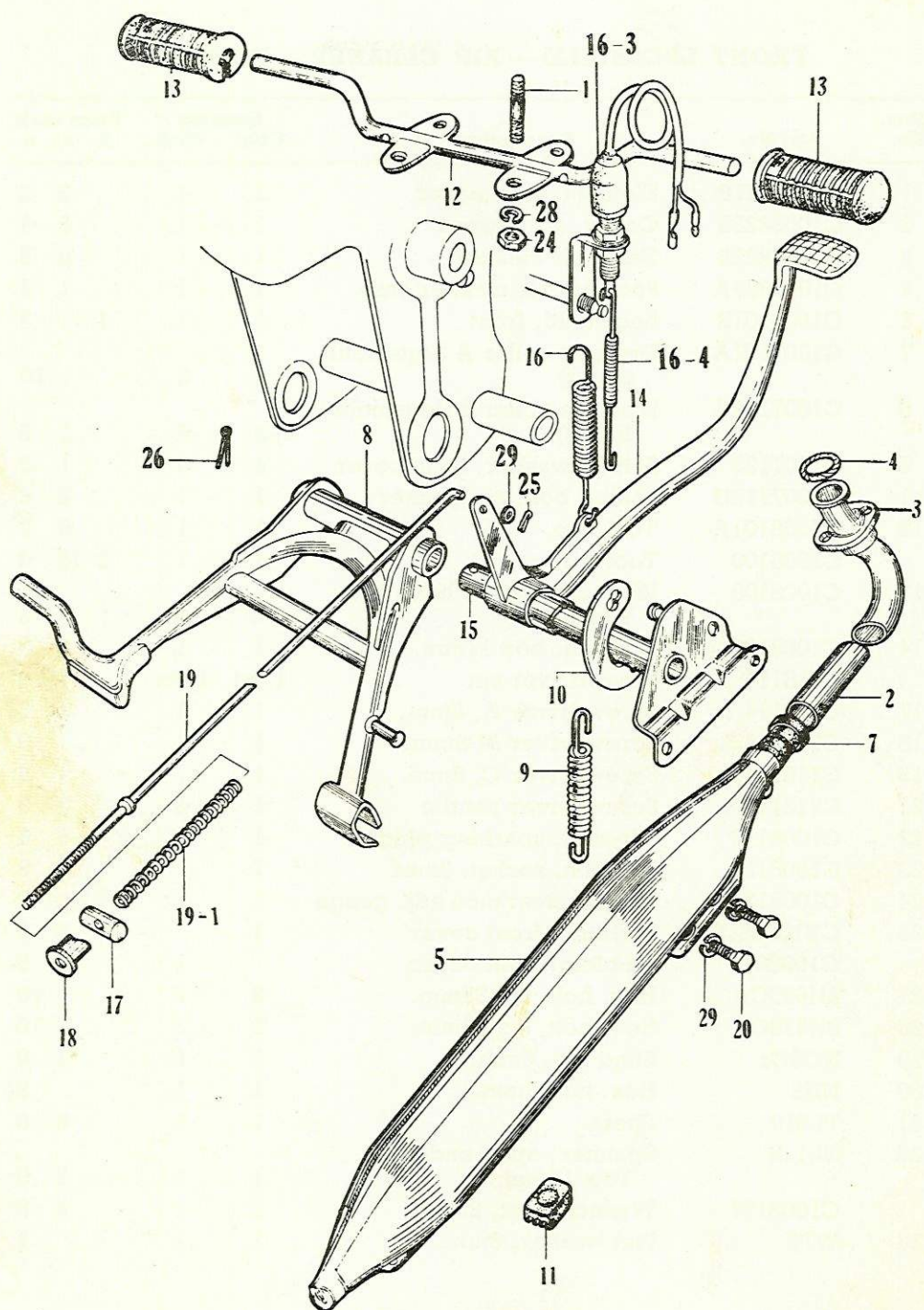
CENTRE STAND — MUFFLER — BRAKE PEDAL
