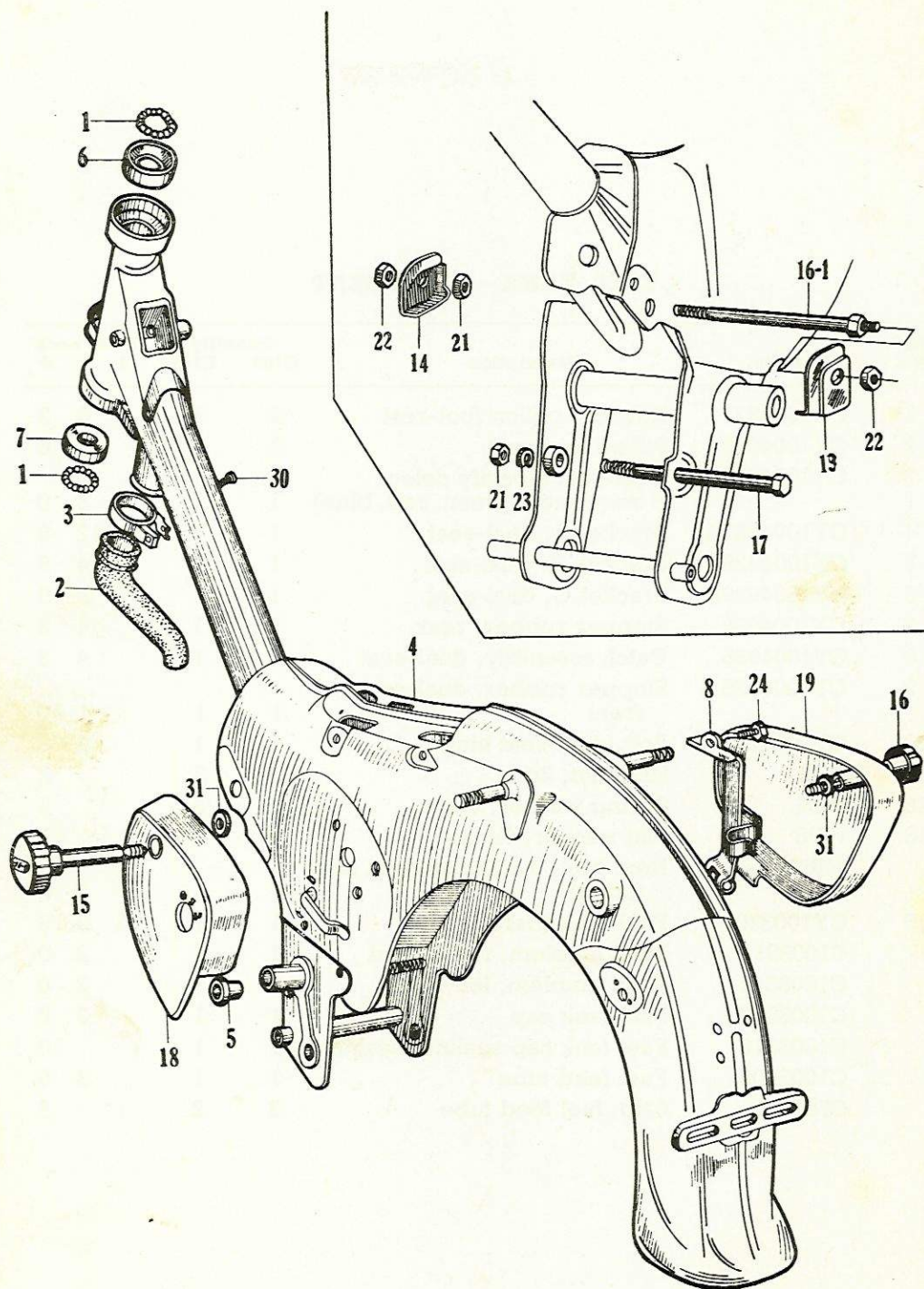
FRAME
