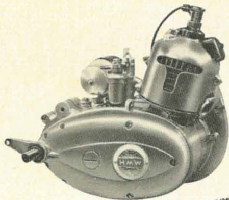
Mk 50 N3G moped engine
