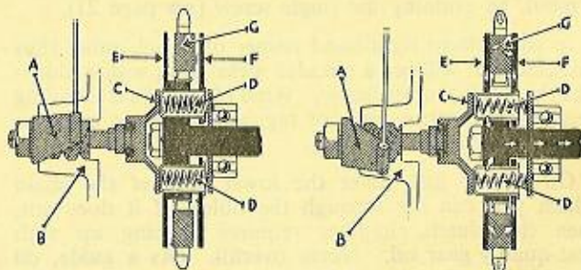
CLUTCH "OUT"
