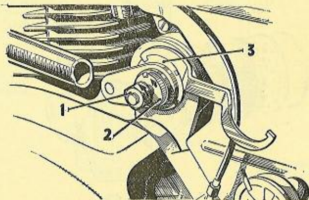
How to adjust the chain from the clutch shaft to the drum.
