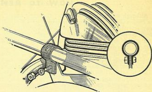
The correct fixing of the bracket which secures the engine to the forks is very important (see page 6).
