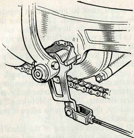
The linkage, for the back-peddalling rear brake, which should periodically be lubricated.
