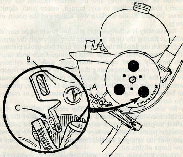
Adjustment of the contact-breaker points on units employing Wico-Pacy magnetos is effected through the marked inspection hole. Loosen the screw A, when the plate B can be moved to alter the gap C.
