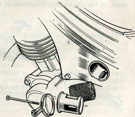
Three stages in the removal of the "Quickly's" air filter, which is built in the frame.
