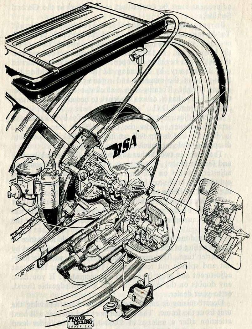
The 35 c.c. B.S.A. "Winged Wheel."
