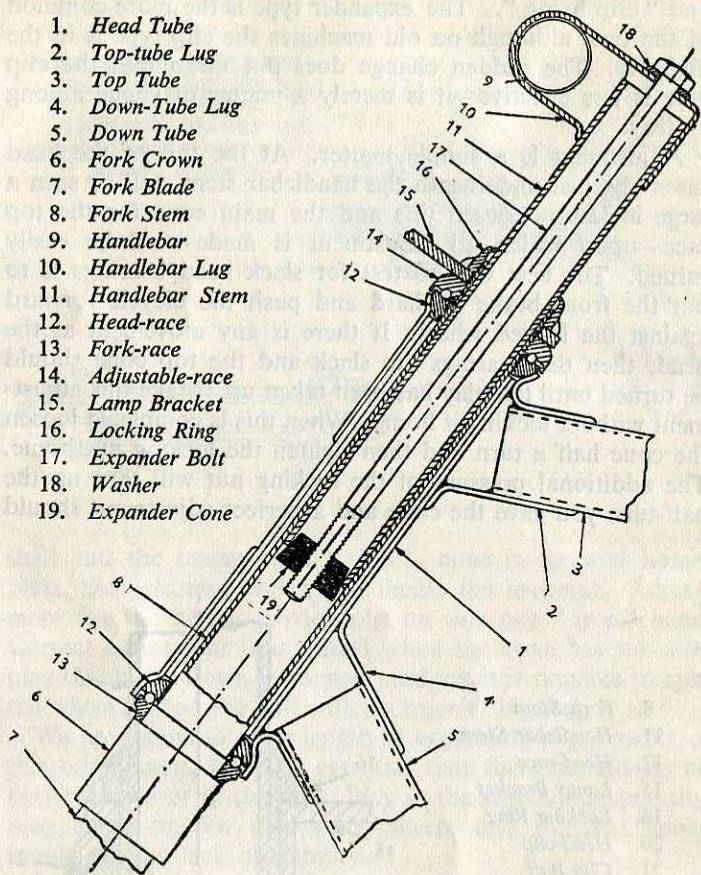
Standard on most modern cycles is the expander-type of steering head assembly, seen here in section.
