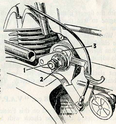
Chain adjustment on "Cyclemaster" units is effected, as shown, by means of a C-spanner, nut 1 and ring 2 first being loosened.
