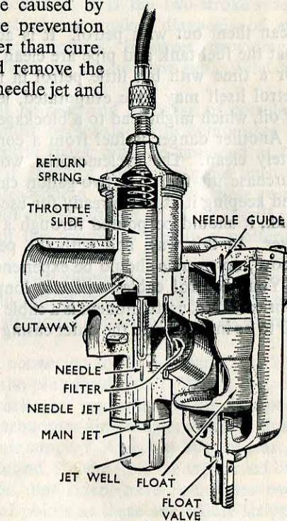
The special Amal carburetter employed on many British cycle-motors.
