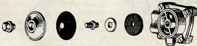
This simple membrane pump, operated by variations in crankcase pressure, supplies fuel to the carburetter on the "VeloSolex". It contains a filter.
