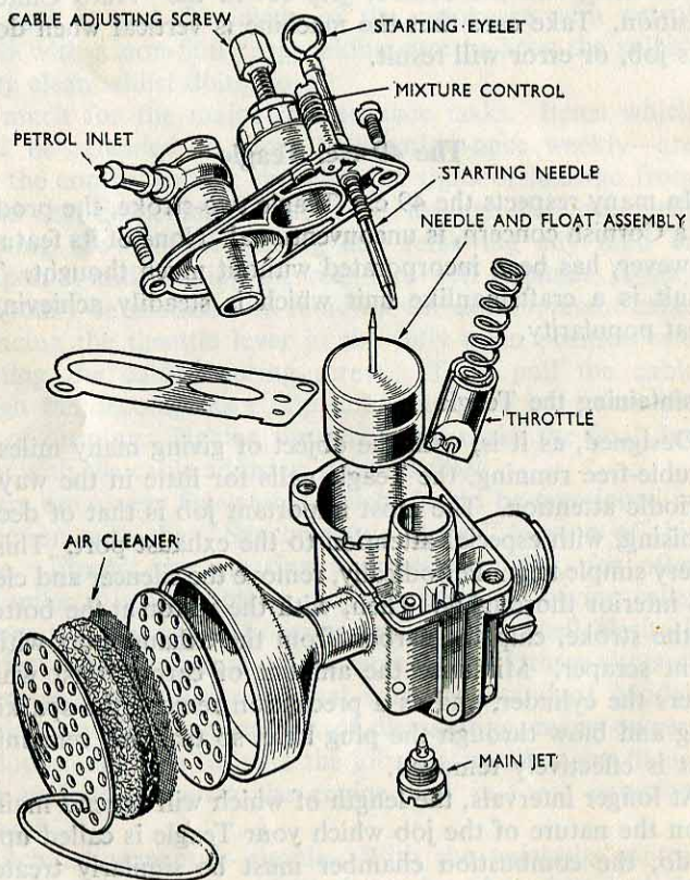
Internal details of the B.E.C. carburettor are clearly shown in this drawing.
