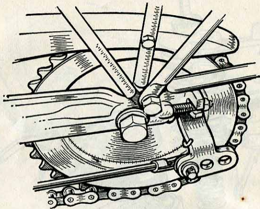
Three alternative rod positions are provided on the "Quickly", permitting adjustment
