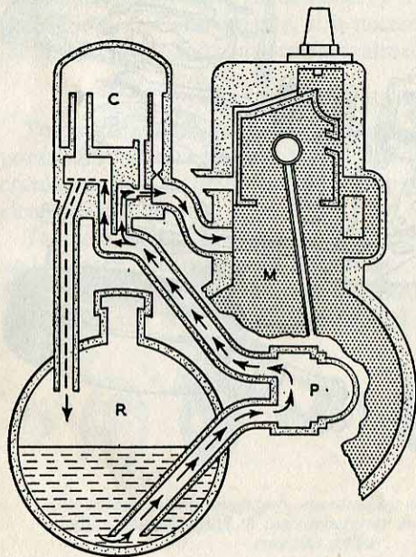
A diagrammatic explanation of the "Velo-Solex" fuel system. Fuel is pumped to the carburetter, any excess being returned by gravity to the tank.
