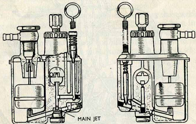
Two sections through the B.E.C. instrument, showing the arrangement of the jets and various passages.
