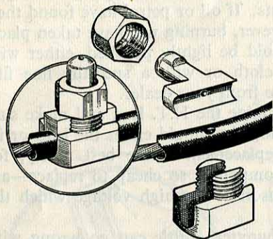
Lubrication of control cable is facilitated by the use of a Kirk cable lubricator shown here.
