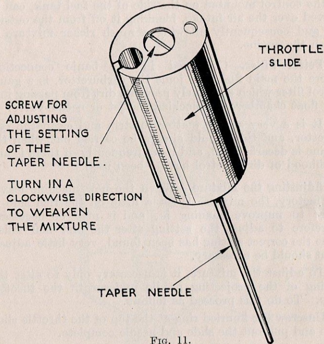
FIG. 11. THROTTLE SLIDE.
