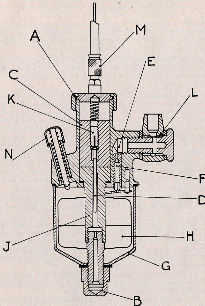
FIG. 10. VILLIERS CARBURETTOR.
