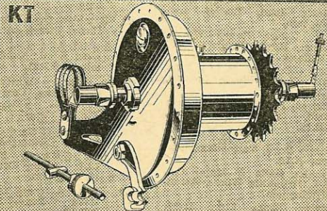
KT 3-speed, 33% increase, 25% reduction.
