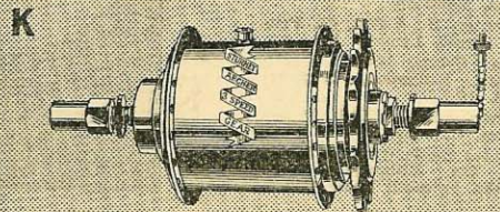
K 3-speed, 33% increase, 25% reduction.
