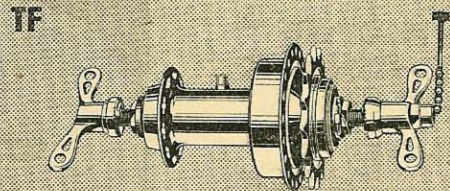
TF 2-speed, 25% reduction.
