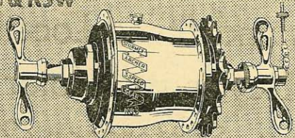
KS. Close ratio 3-speed, 12.5% increase, 11.1% reduction. KSW. Medium ratio 3-speed, 16.6% increase, 14.3% reduction.
