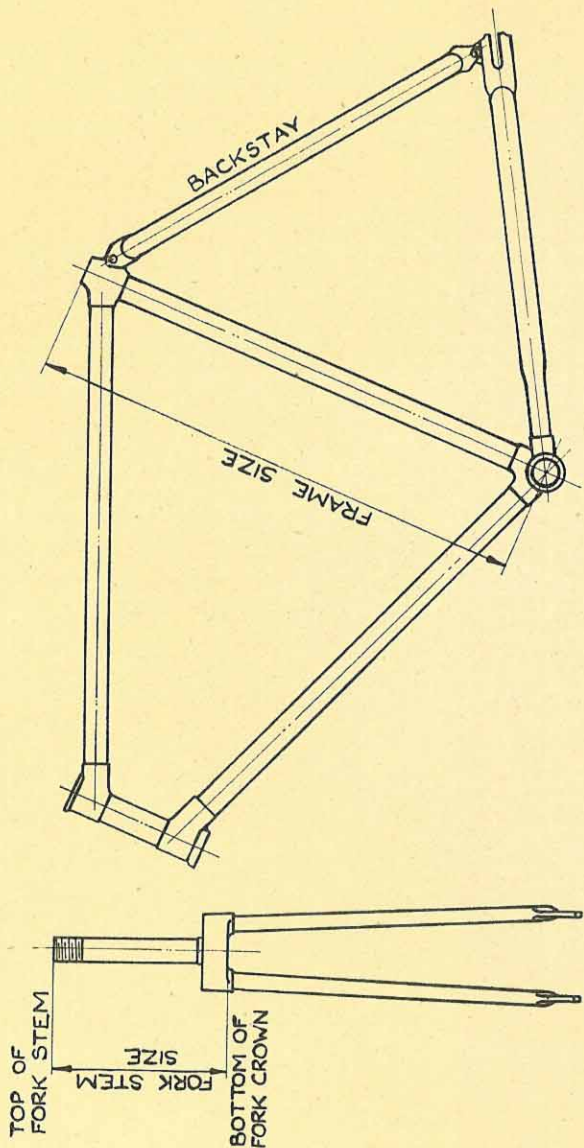
FRAME AND FORK DIMENSIONS
