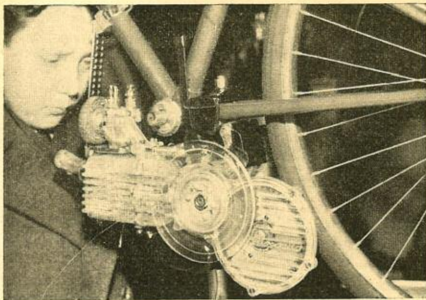
Showing the internals—a 48 c.c. Mosquito cycle attachment with plastic flywheel, covers, and other components
