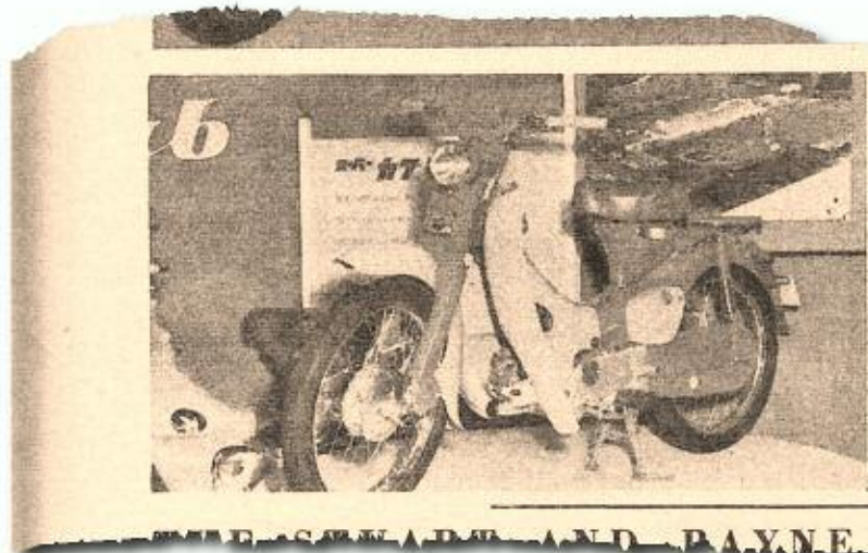
(Left) The Super-Cub, with a 90 c.c. o.h.v. engine, almost horizontally disposed, is an ultra-lightweight open-frame motorcycle in which pressed steel is widely used.
