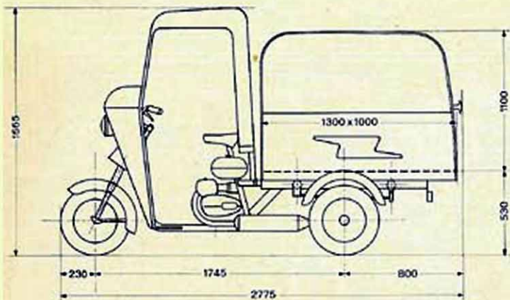
PRESSED STEEL CLOSED VAN "GIARDINETTA" - Opening of the rear little doors: mm. 810 x 810 (ft. 2.6575 x 2.6575)
