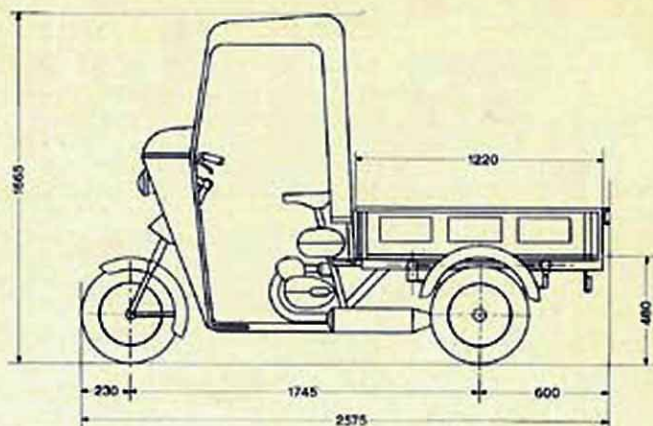
NORMAL PRESSED STEEL PLATFORM - Inner sizes: mm. 1180 x 950 x 250 (ft. 3.8713 x 3.1168 x 0.8202)
