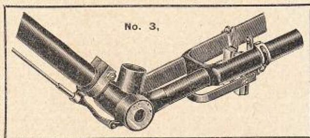
Patent Double Bearing Clip, providing a straight and rigid pull under Bottom Bracket in connection with Back Rim Brake.
