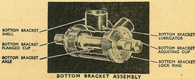
BOTTOM BRACKET ASSEMBLY
