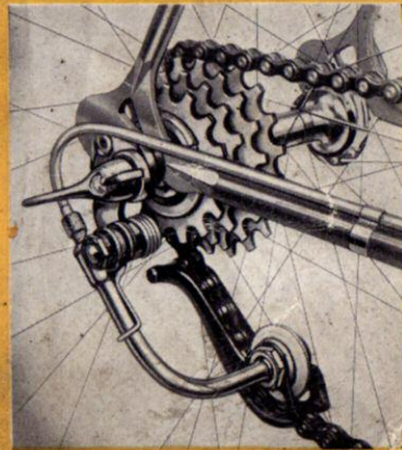
B.S.A. 4-Star Gear
